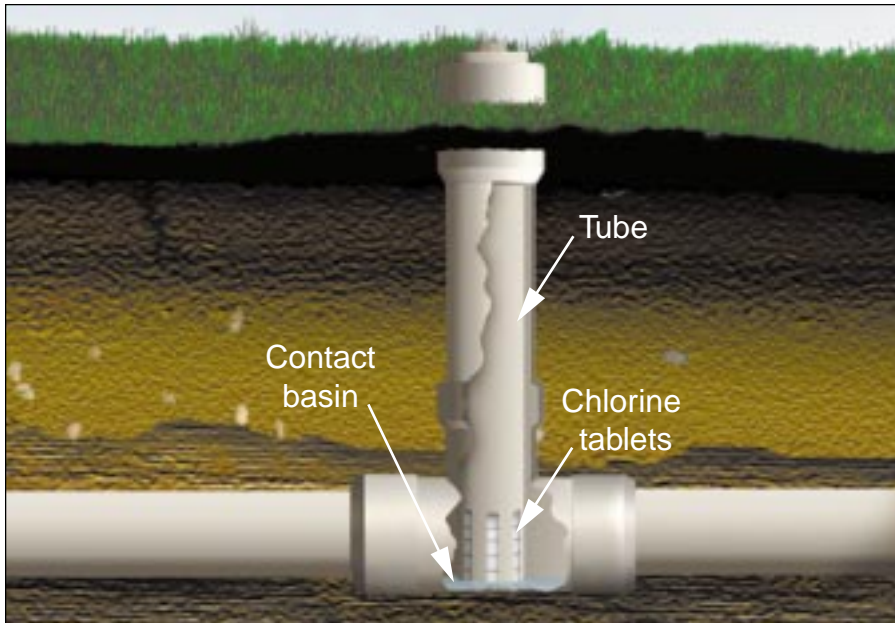
Figure 2: Wastewater disinfection begins in the contact basin.
